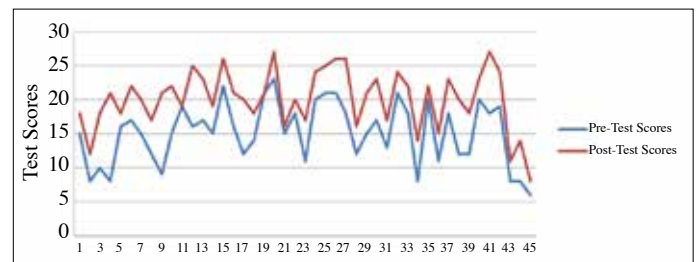
Figure 1. Comparison of pre-test and post-test scores
